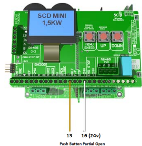
Schema Doorcontrol V7
